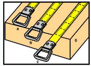
Zero points of tape measures (a) Standard, (b) Excluding hook and (c) 10 cm Blank
